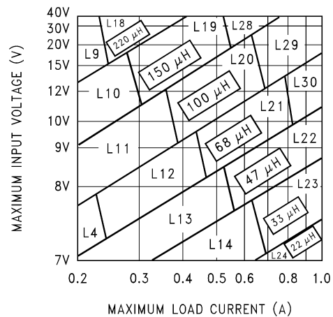
Figure 23. LM2595-5.0
