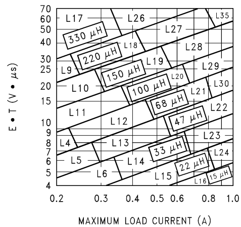
Figure 25. tLM2595-ADJ
