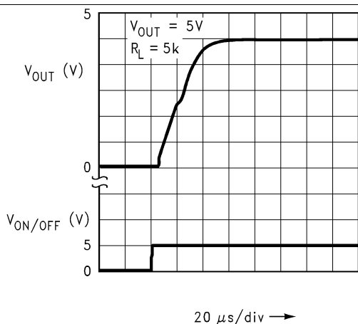
Figure 29. Turn-On Waveform
