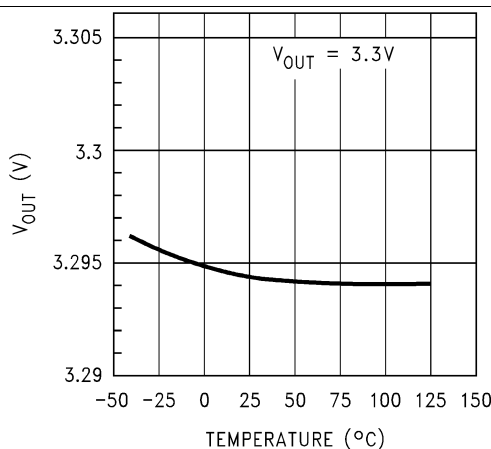
Figure 2. 3.3-V Output Voltage vs Temperature
