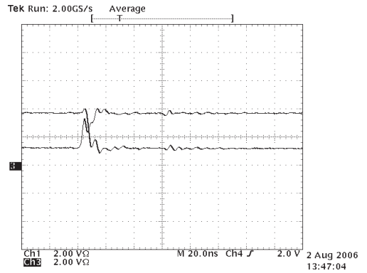
Driver Output Waveform Low to High
