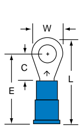
MV14-10R Stud Size 10 Wire Range 16-14
