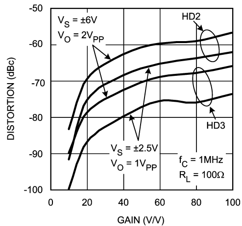
Distortion vs. Gain
