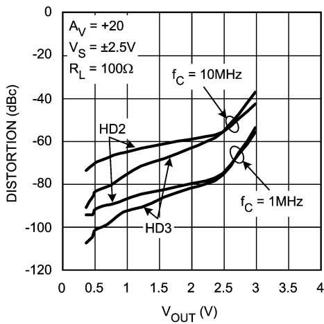
Distortion vs. V_{OUT} Peak to Peak
