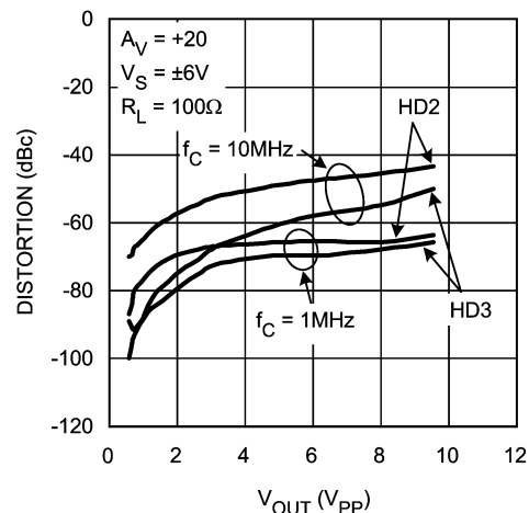
Distortion vs. V_{OUT} Peak to Peak
