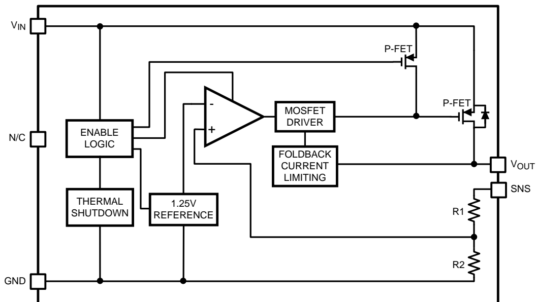
Figure 5. LP38691 Functional Diagram (WSON)
