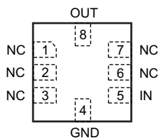
Pin Functions
