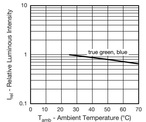
Fig. 18 - Relative Luminous Intensity vs. Ambient Temperature
